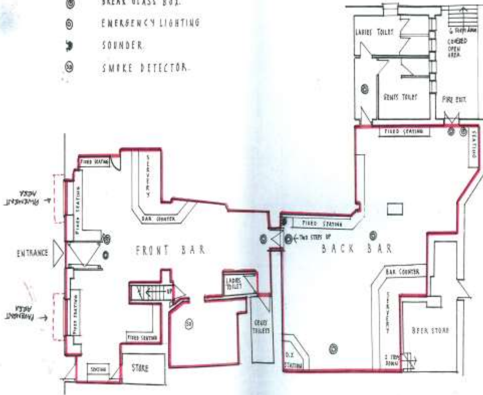
ANGEL INN UPPER GT DARKGATE ST ABERYSTWYTH. GROUND FLOOR LAYOUT. SCALE: 1:100
