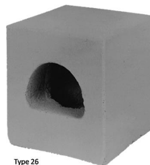
Ffigur D3-10: Blwch bric blaen agored
