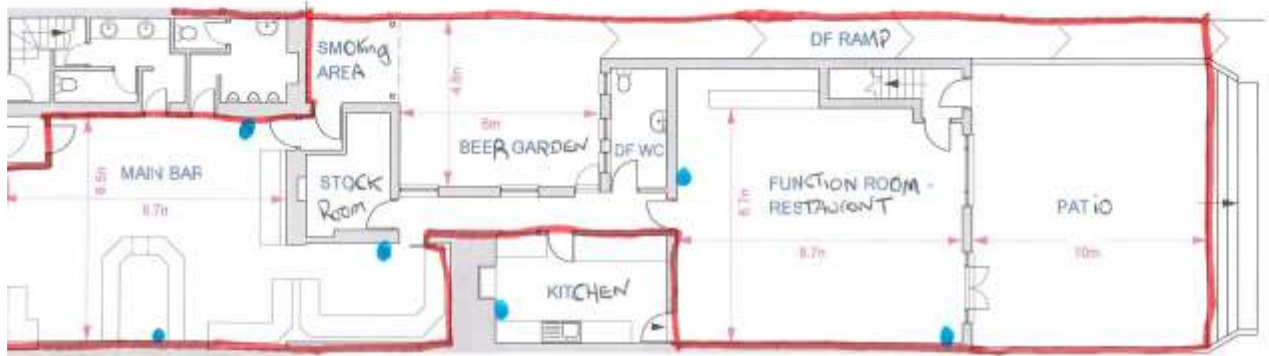
GROUND FLOOR LAYOUT
