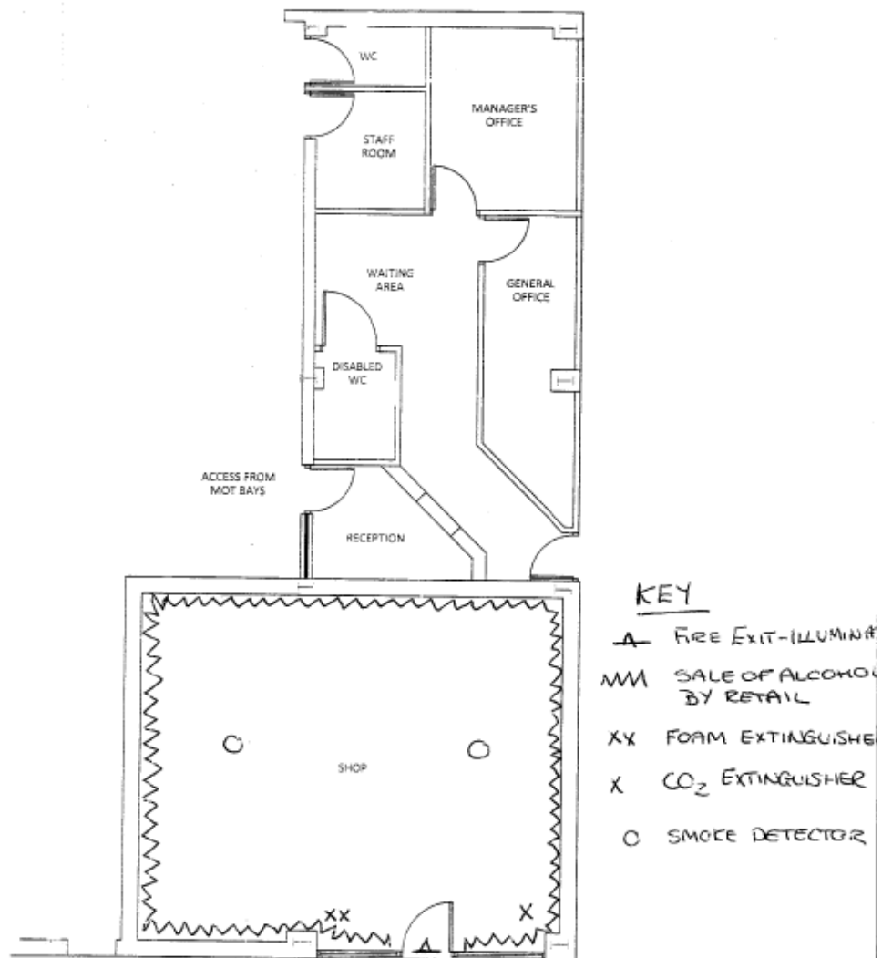
LAYOUT MODIFICATION TO OFFICE FACILITY AT ROBERT DAVIES MOTORS, LLECHRYD
